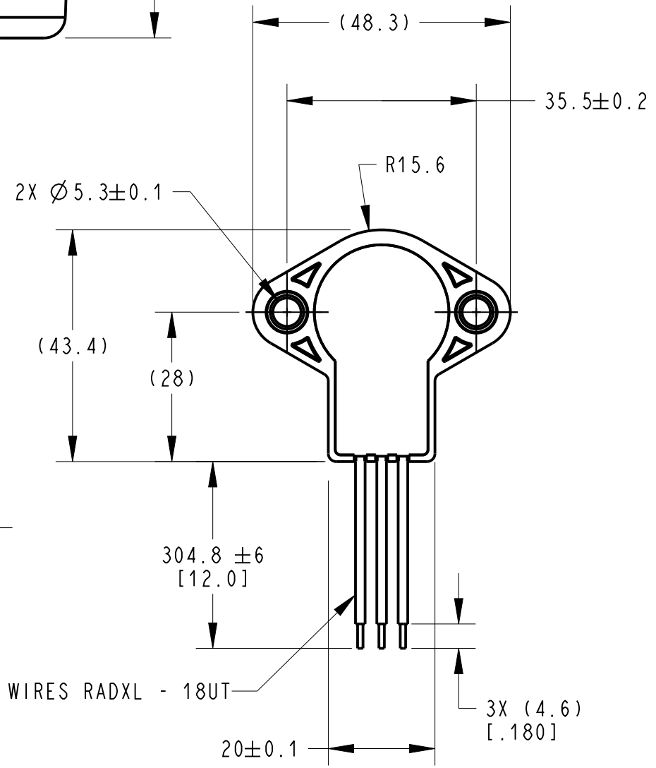
DETAIL B SCALE 4:1
