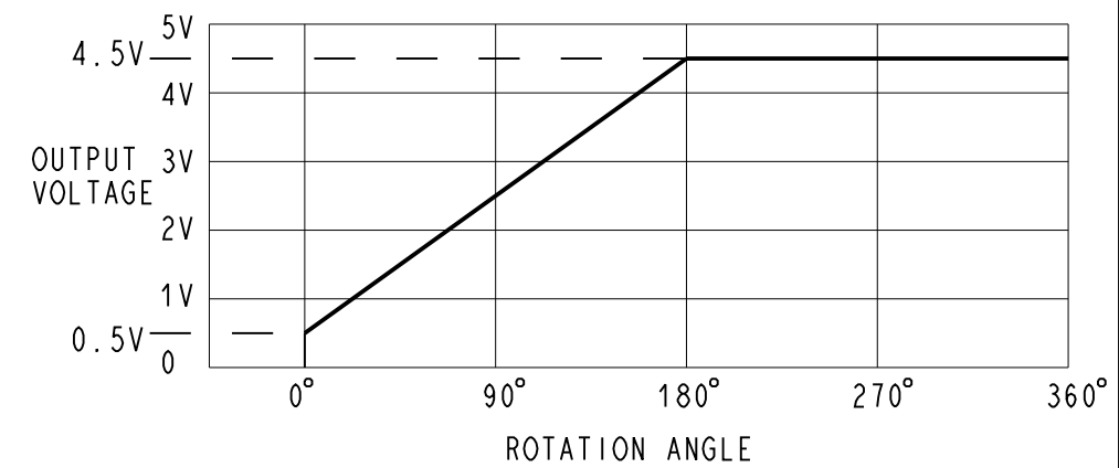
SENSOR OUTPUT SIGNAL (TYPICAL BASED ON 5V SUPPLY)
