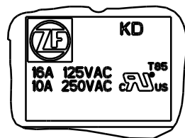
DETAIL A SCALE 3:1
