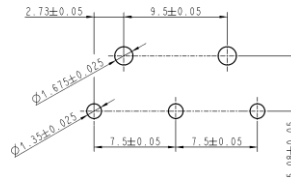
Drilling pattern
