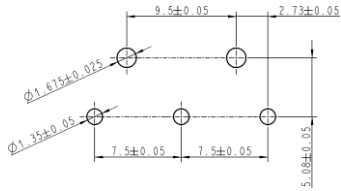
Drilling pattern
